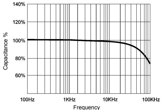
Typical Component Capacitance vs. Frequency
