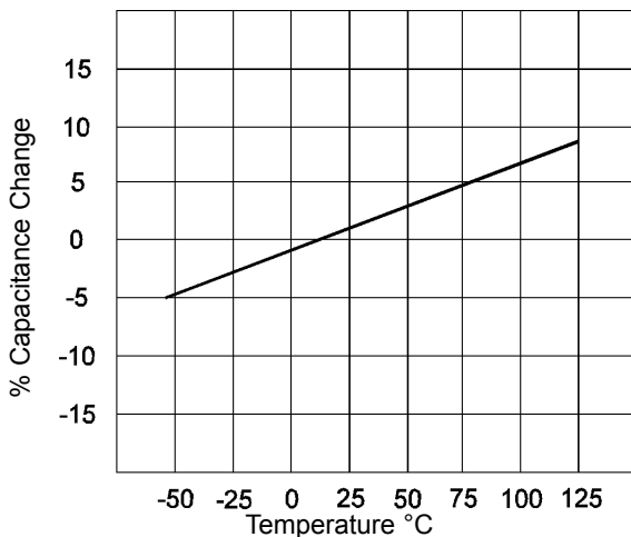
Typical Component Capacitance vs. Temperature
